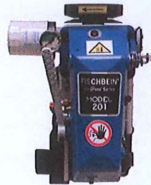
Head 201 for tape sewing: possibility to sew with or without crepe paper
